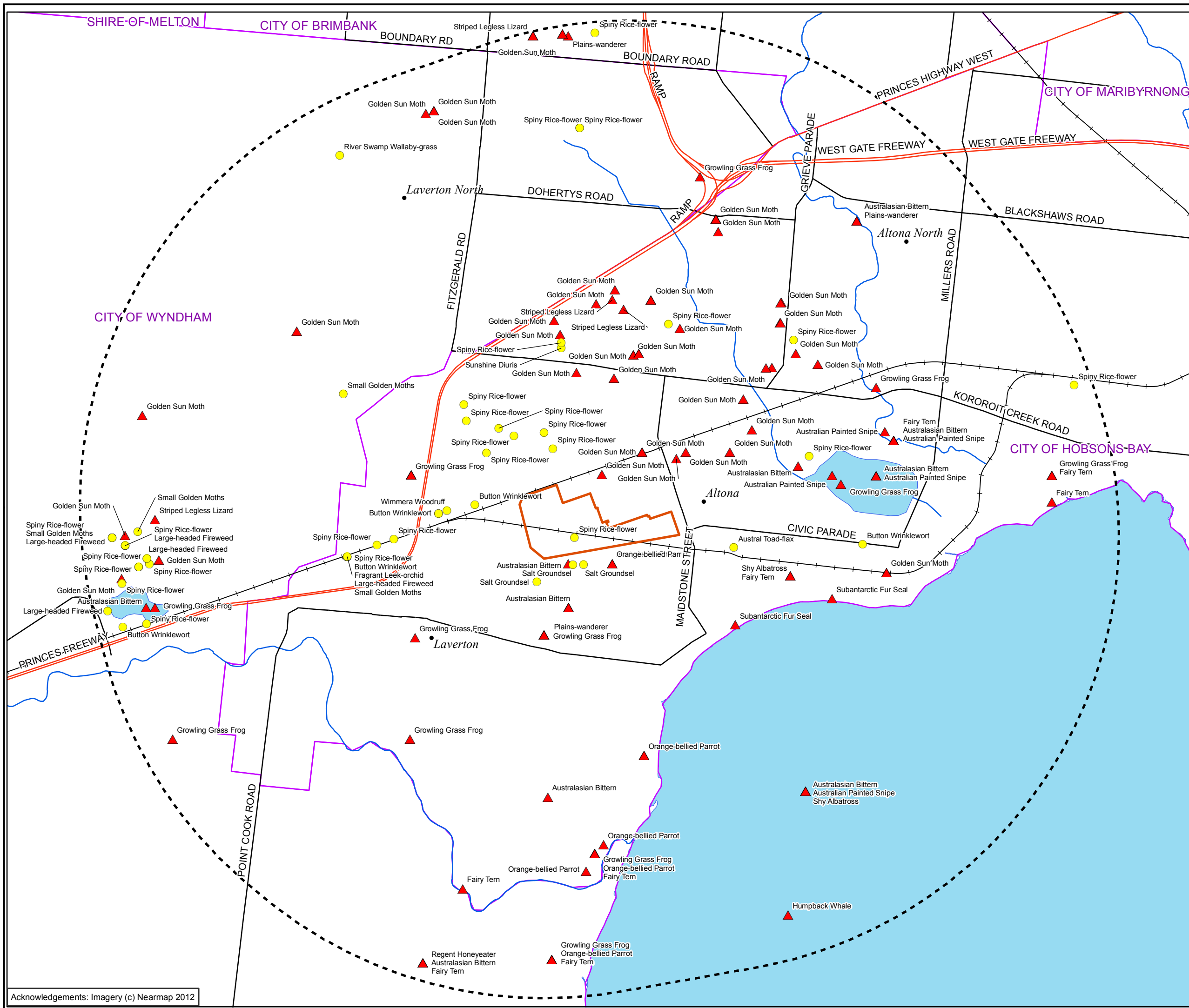
Figure 4: EPBC listed flora and fauna species within 5km of the Ajax Road properties, Altona
