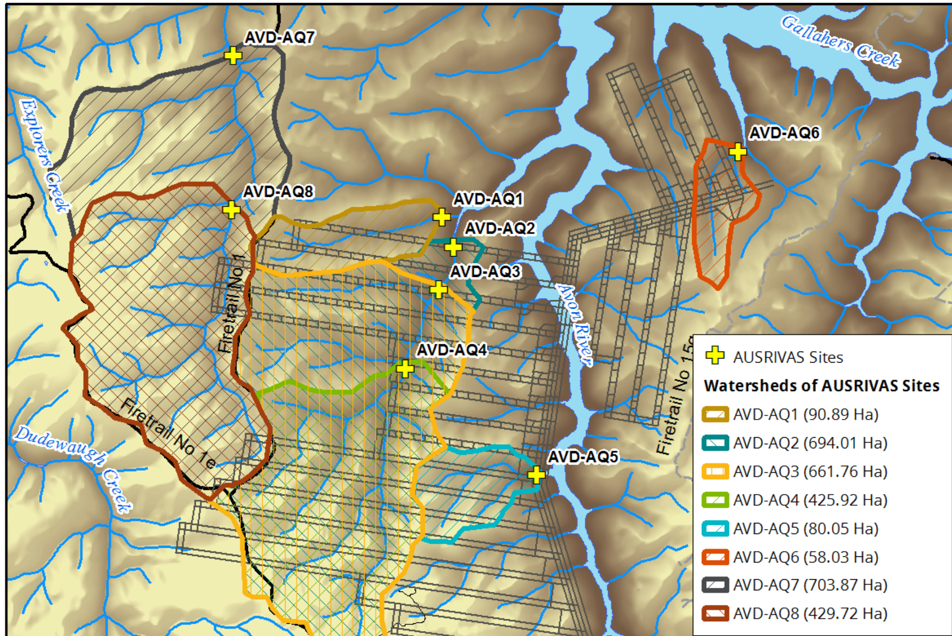
Figure 3: Example of Aquatic Monitoring Site Catchment Modelling
