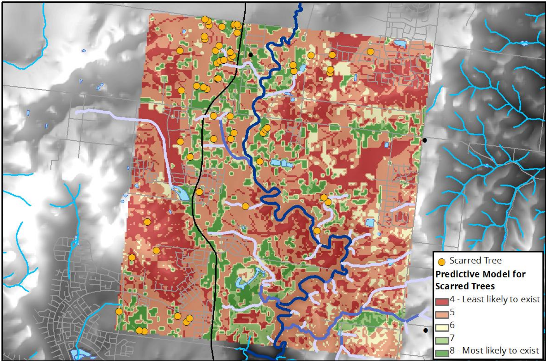
Figure 2: Example of Aboriginal Heritage Predictive Modelling Using Weighted Overlay Analysis
