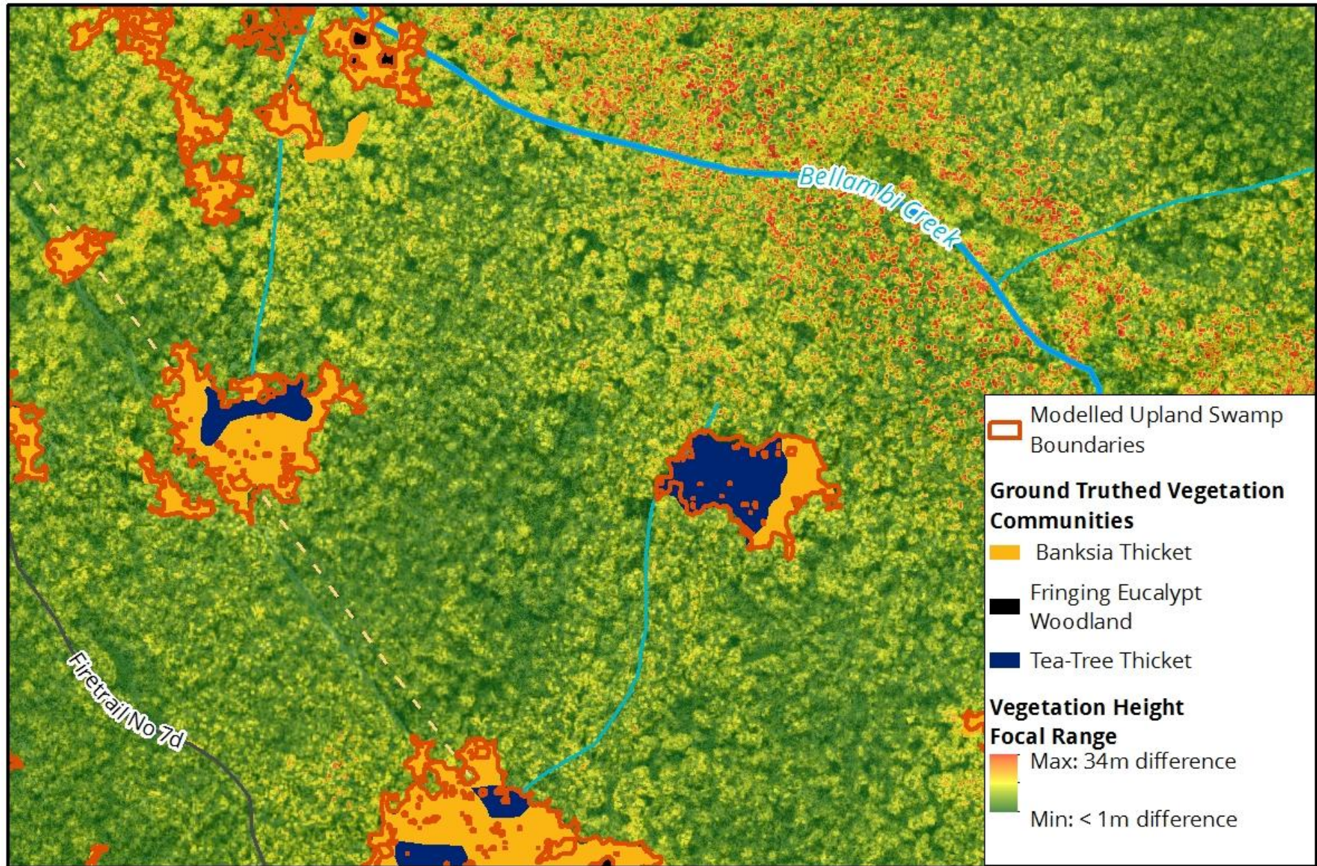
Figure 1: Example of Coastal Upland Swamp Modelling to Monitor the Effects of Mining Subsidence on Threatened Ecological Communities
